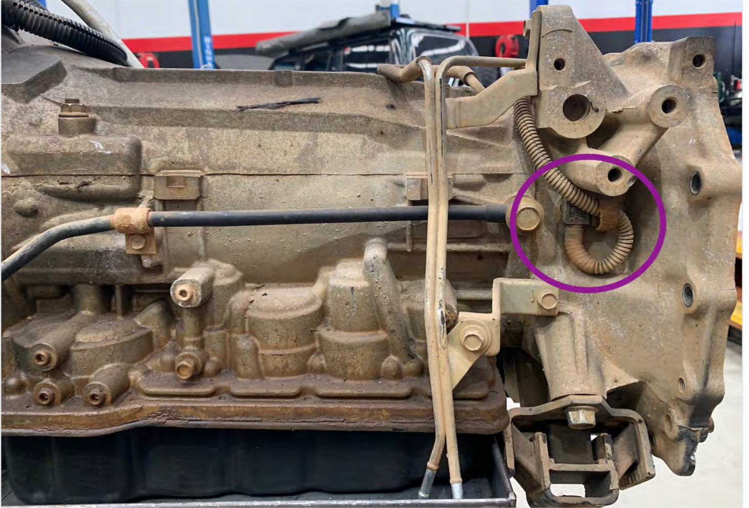
Internal Loom Lever Switch
